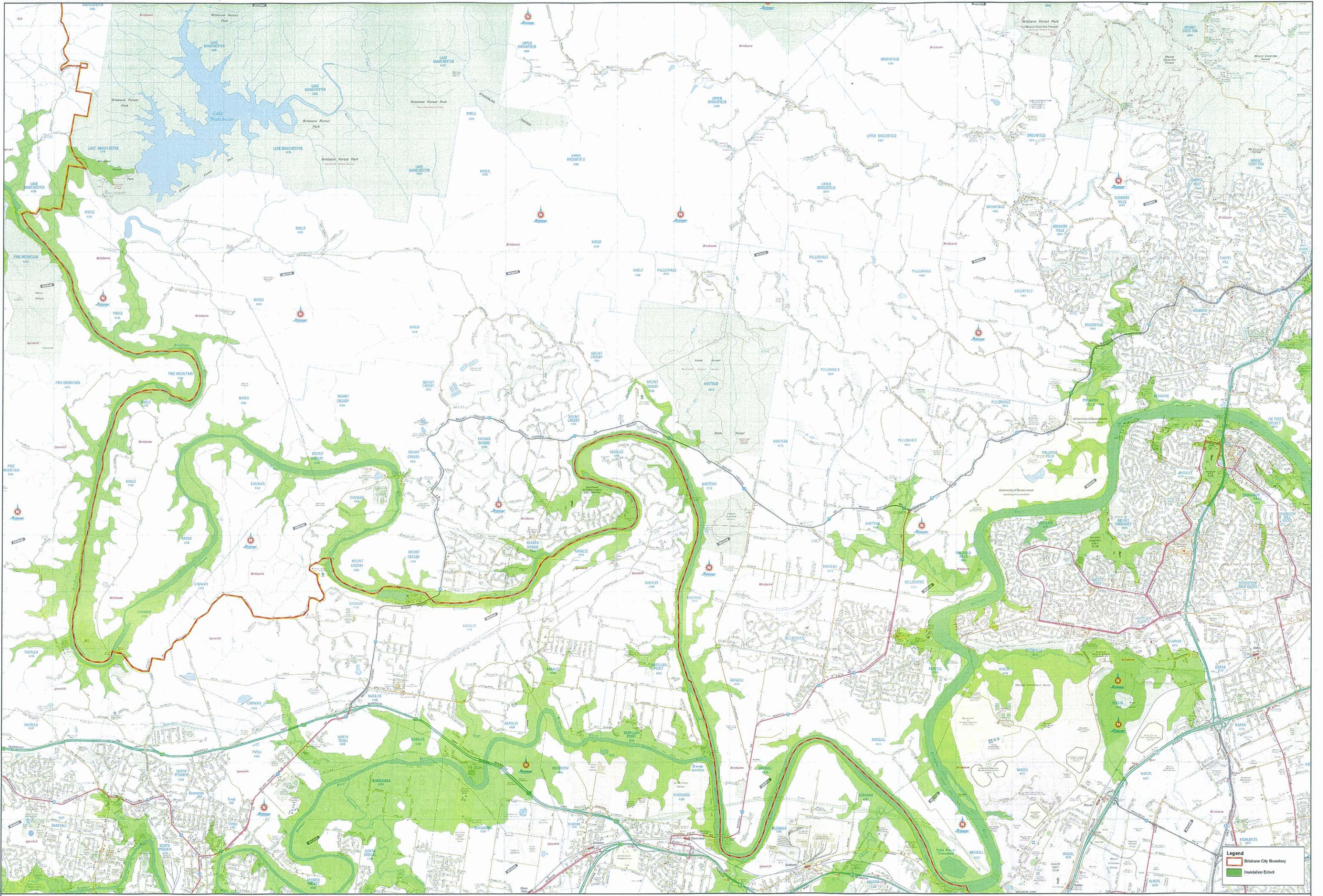
7,000 m 3 /s Peak Discharge at Port Office Gauge Inundation Extents - West
