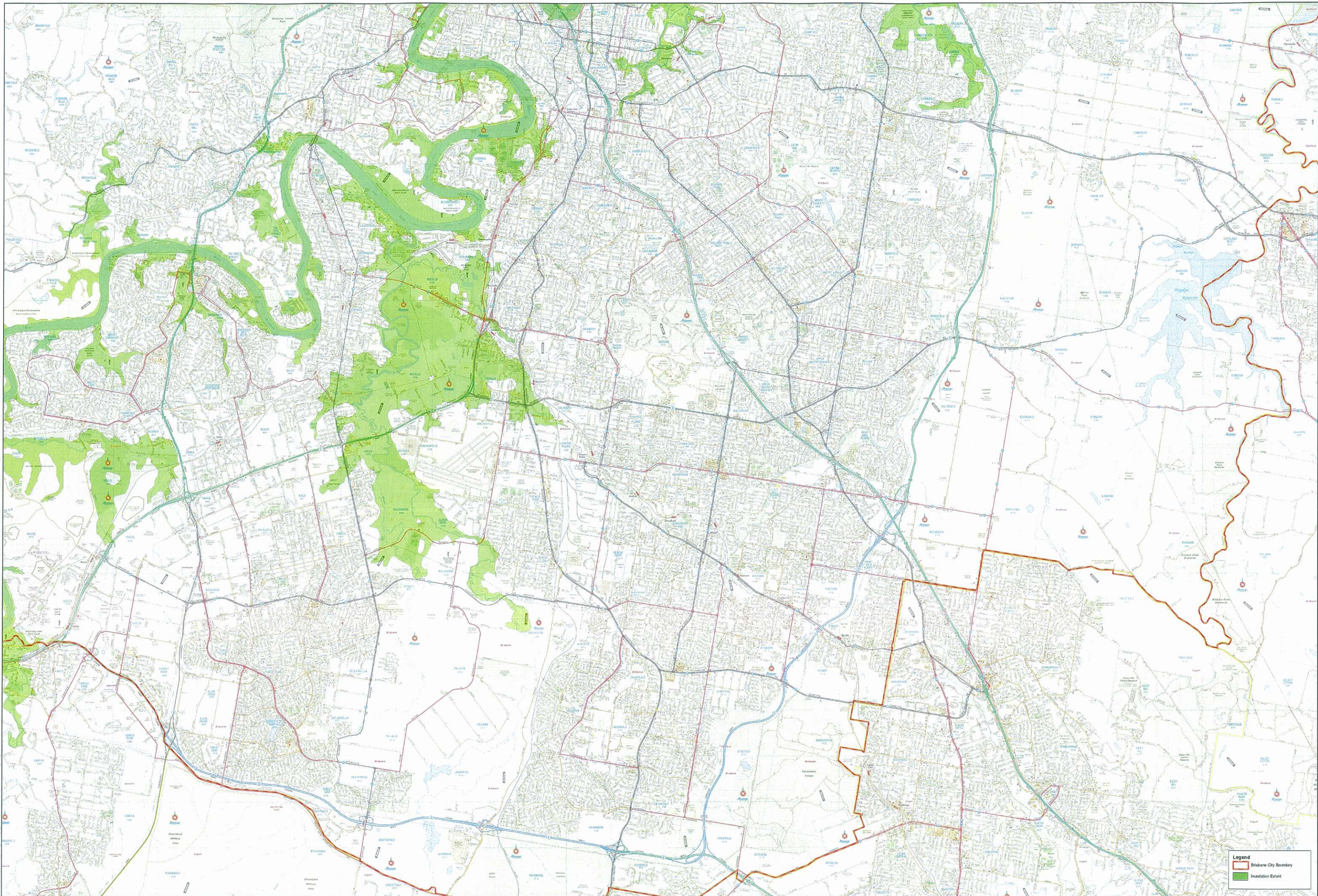
7,000 m 3 /s Peak Discharge at Port Office Gauge Inundation Extents - South
